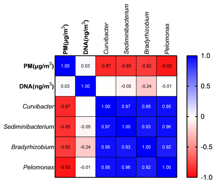
Fig. 5. Correlations between particulate matter (PM) and genera (or metagenomic DNA). Among the major genera, only four genera showed a significant correlation with PM.
