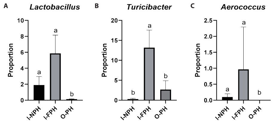
Fig. 3. Microbiome profiles in particulate matter collected inside and outside of the pig house. a,b Different superscript letters indicate significant differences. I-NPH, inside the nursery pig house; I-FPH, inside the finishing pig house; O-PH, outside of the pig house.
