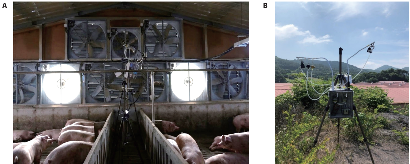
Fig. 1. Measurement of particulate matter (PM) inside and outside the pig house. (A) PM sampling inside the pig house. (B) PM sampling outside the pig house.
