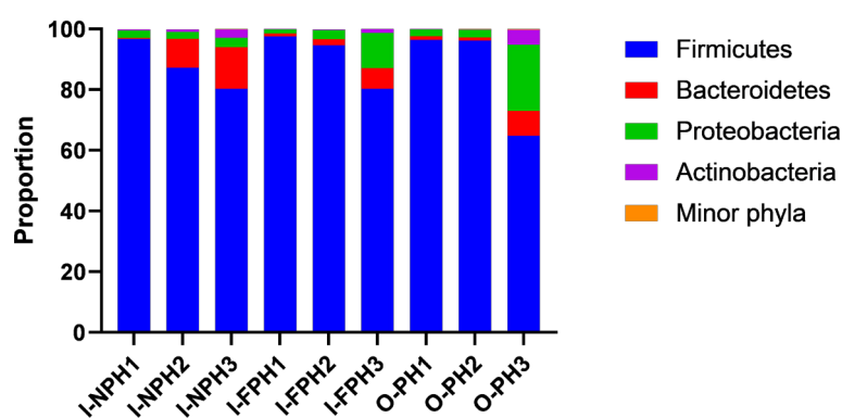
Fig. 2. Microbiome profiles in particulate matter collected inside and outside of a pig house. I-NPH, inside the nursery pig house; I-FPH, inside the finishing pig house; O-PH, outside of the pig house.
