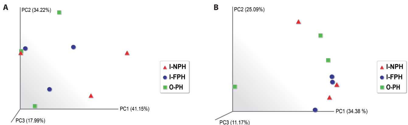
Fig. 4. Weighted (A) and unweighted (B) principal coordinate analysis indicating similarity among the three groups of particulate matter (PM) samples. Microbiomes of the three sampling groups were not separated. NPH, inside the nursery pig house; I-FPH, inside the finishing pig house; O-PH, outside of the pig house.
